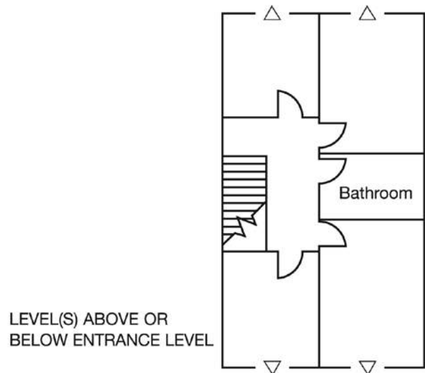
Figure 6 – Multi storey flat with alternative exits, from each habitable room, except at entrance level
